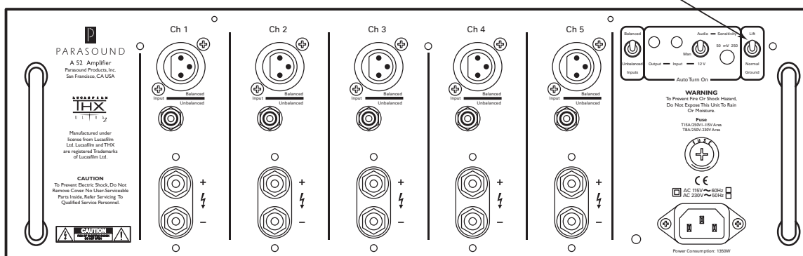
Ground Switch, set to up position
